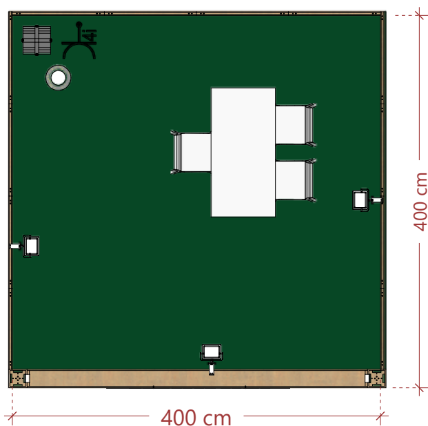
pianta | floor plan*
